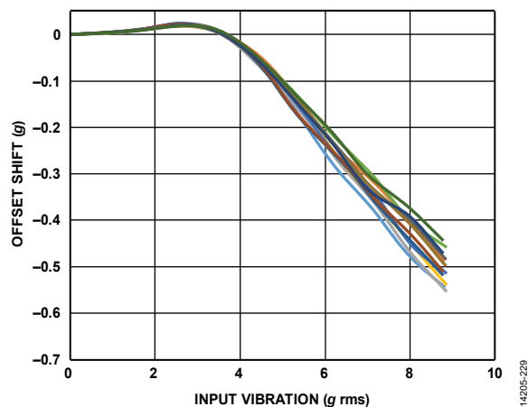
Figure 30. ADXL354 VRE, Y-Axis Offset from +1\text{ g} , \pm 8\text{ g} Range, Y-Axis Orientation = +1\text{ g}
