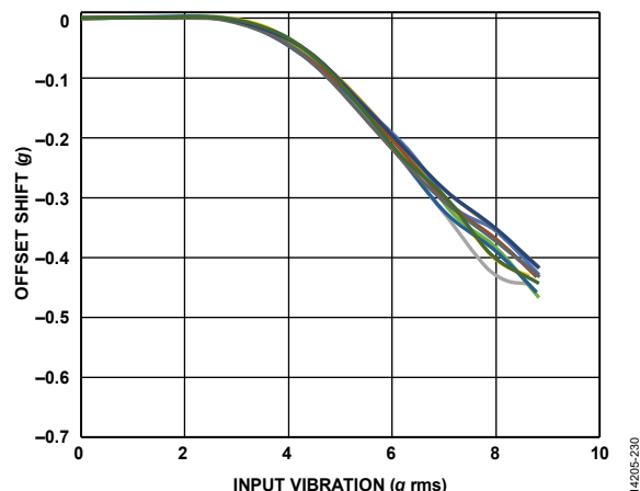
Figure 31. ADXL354 VRE, Z-Axis Offset from +1\text{ g} , \pm 8\text{ g} Range, Z-Axis Orientation = +1\text{ g}
