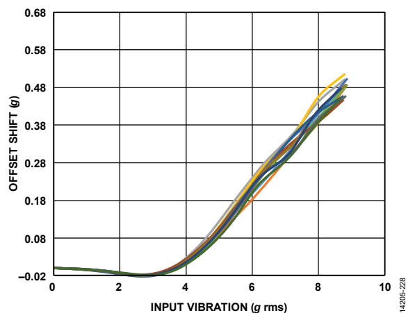
Figure 29. ADXL354 VRE, X-Axis Offset from -1\text{ g} , \pm 8\text{ g} Range, X-Axis Orientation = -1\text{ g}
