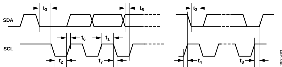
Figure 3. I²C Timing
