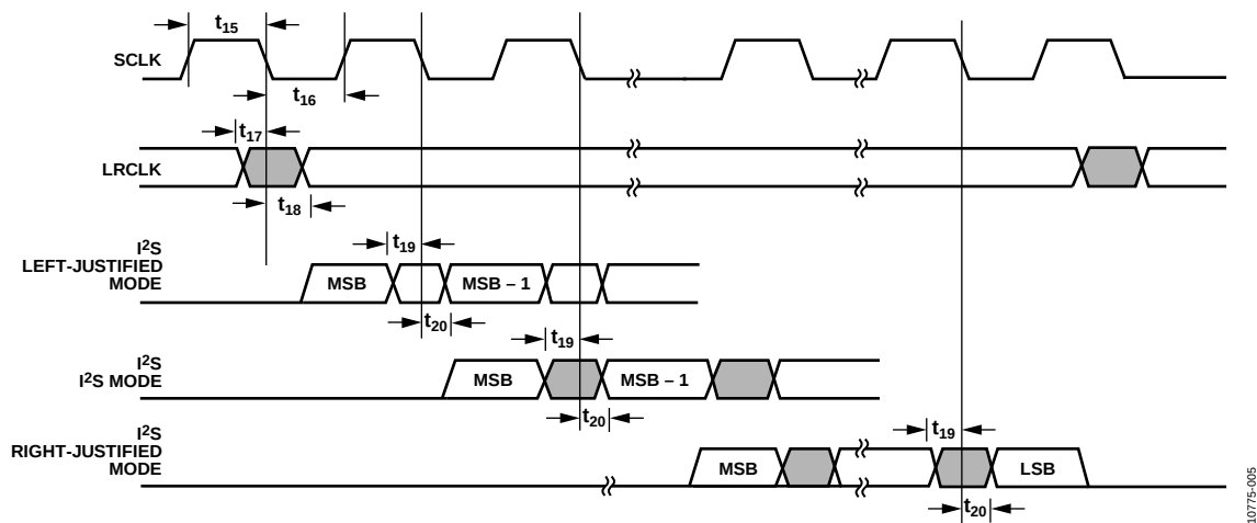
Figure 5. I²S Timing
