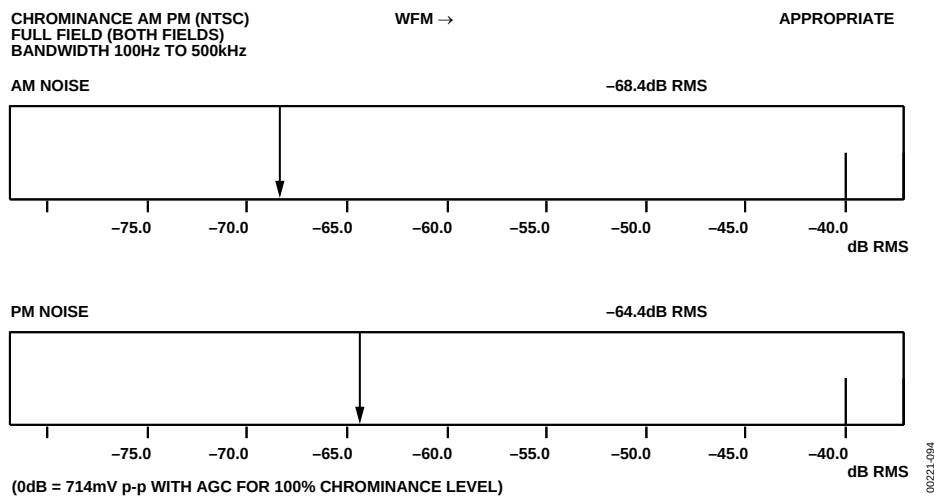
Figure 94. NTSC AM/PM Noise Measurement
