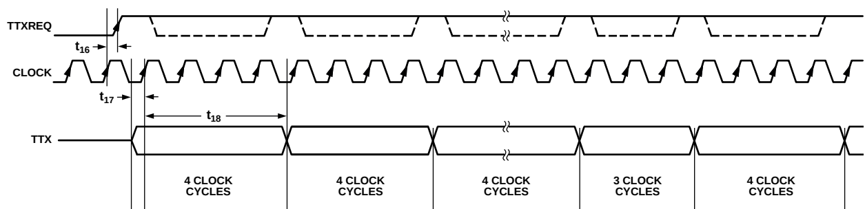
Figure 4. Teletext Timing Diagram
