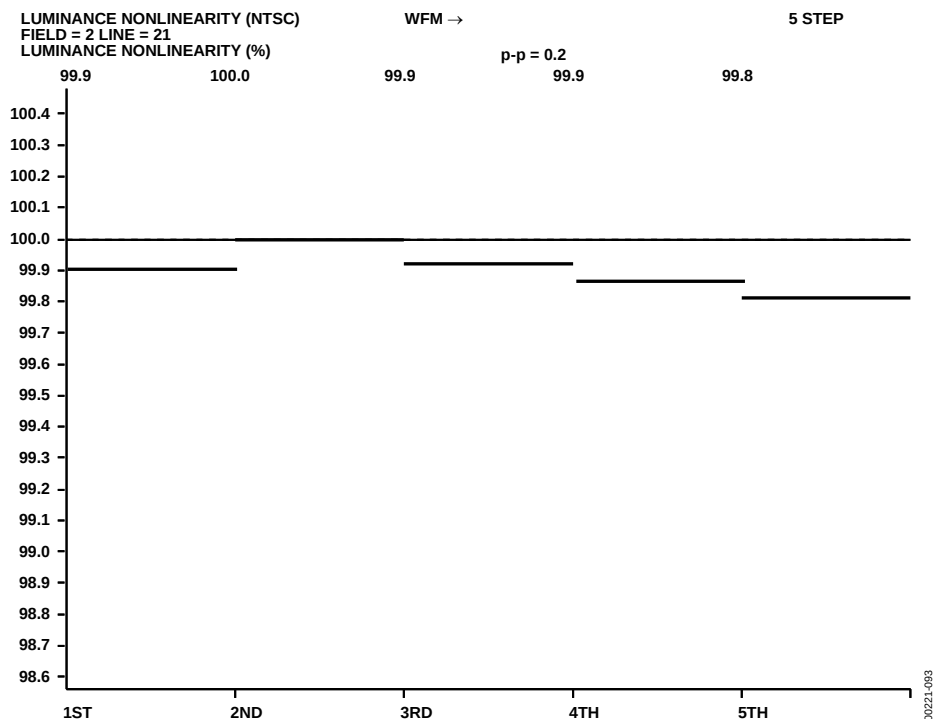
Figure 93. NTSC Luminance Nonlinearity Measurement
