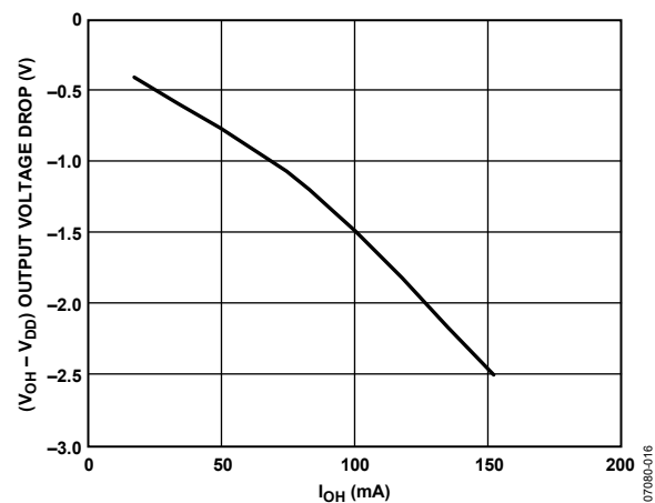
Figure 9. Typical V_{OH} Drop vs. I_{OH} ( V_{DD1} = 5 V, V_{DD2} , V_{ISO} = 12 V to 18 V)
