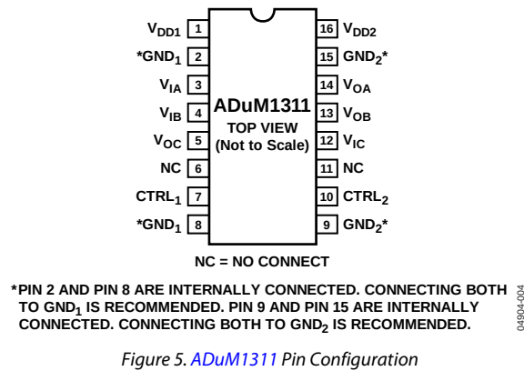
Figure 5. ADuM1311 Pin Configuration
