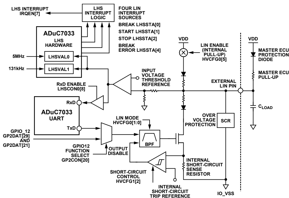
Figure 43. LIN I/O, Block Diagram
