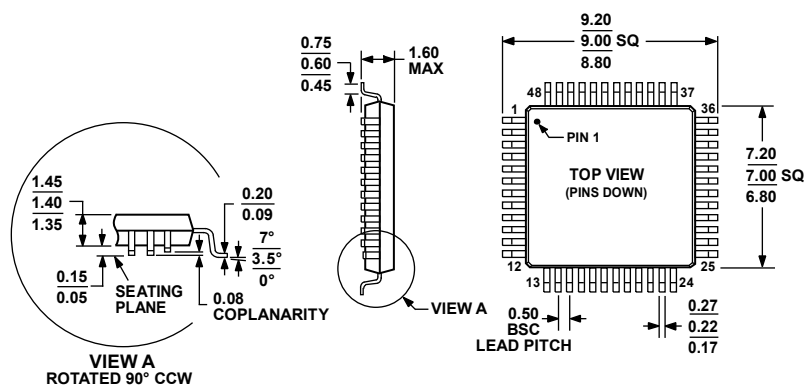
Figure 59. 48-Lead Low Profile Quad Flat Package [LQFP]
