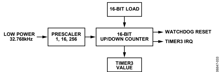
Figure 35. Timer3 Block Diagram
