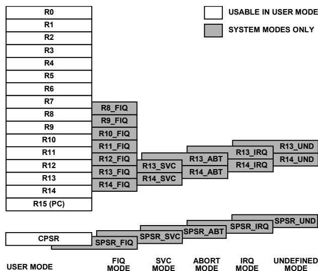
Figure 11. Register Organization
