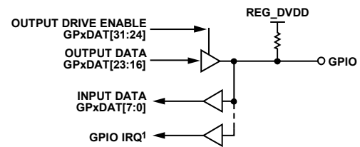
Figure 37. ADuC7033 GPIO
