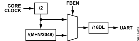
Figure 40. Fractional Divider Baud Rate Generation
