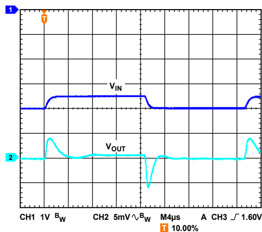
Figure 67. Line Transient Response, 500 mV Step, V_{OUT} = -3\text{ V} , I_{LOAD} = -200\text{ mA}
