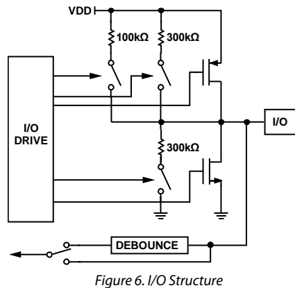
Figure 6. I/O Structure
