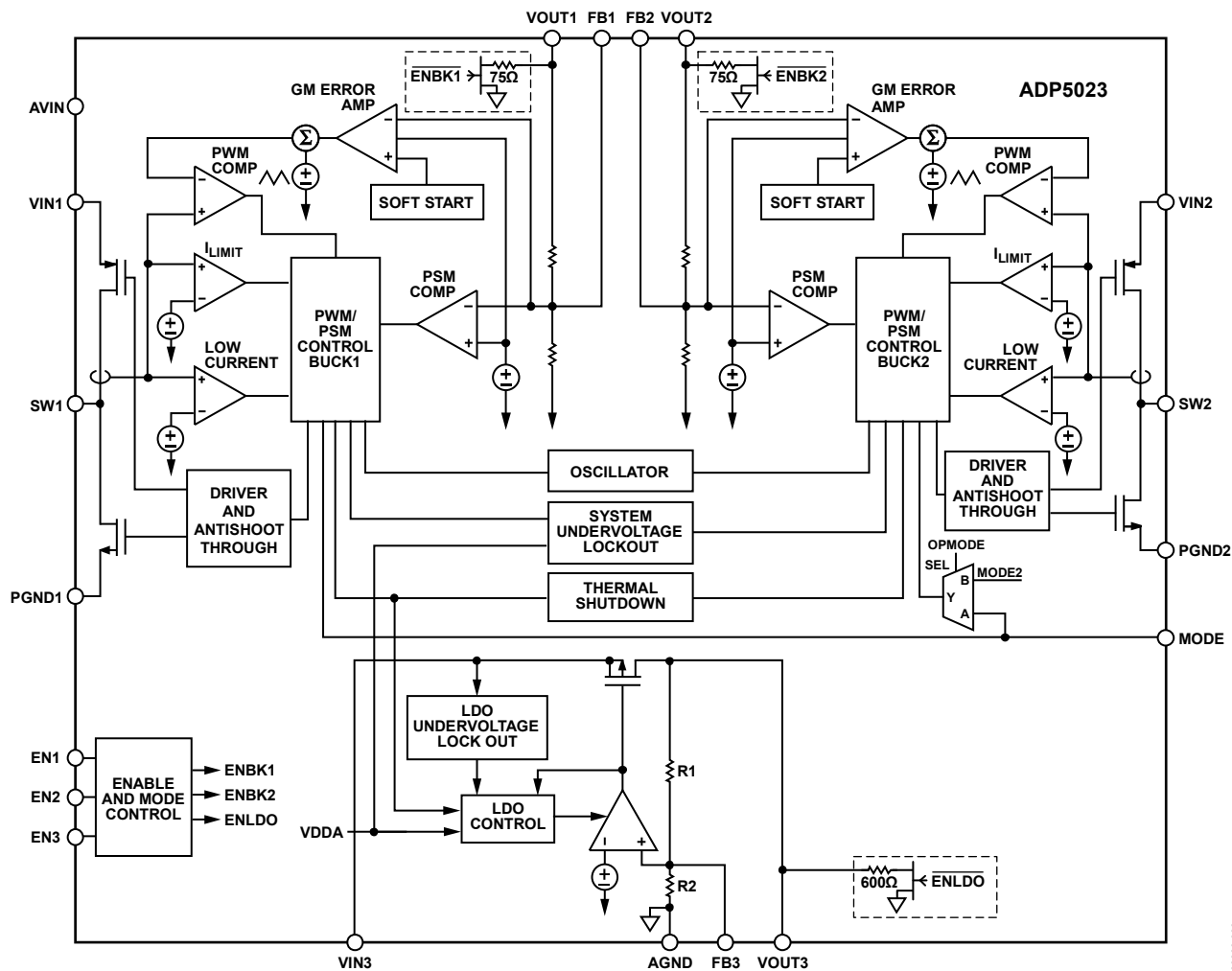
Figure 45. Functional Block Diagram
