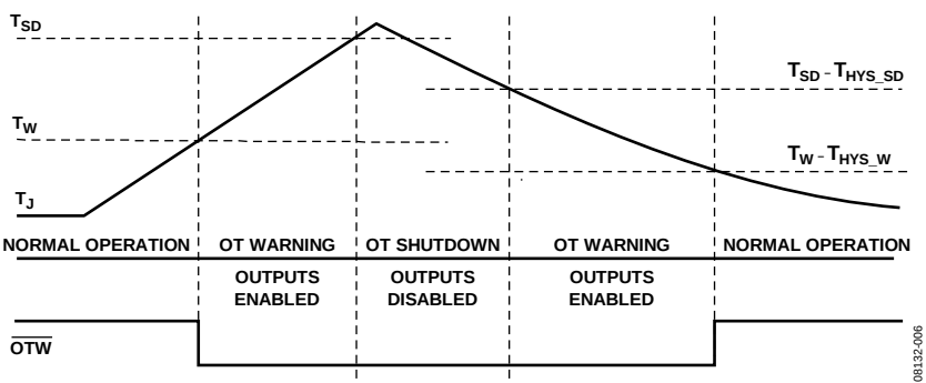
Figure 6. Overtemperature Warning and Shutdown
