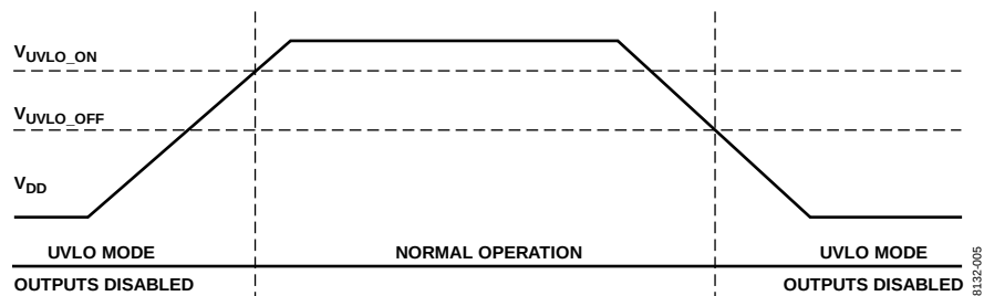
Figure 5. UVLO Function
