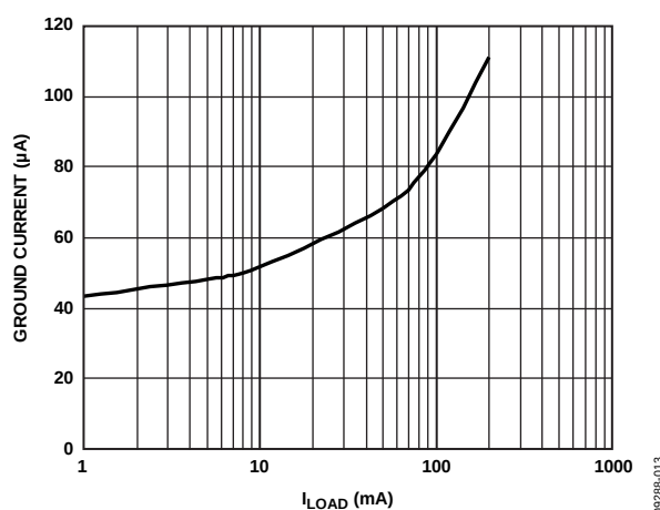
Figure 15. Ground Current vs. Load Current, Single Output Loaded, V_{RIPPLE} = 50\text{ mV} , C_{OUT} = 1\text{ }\mu\text{F}
