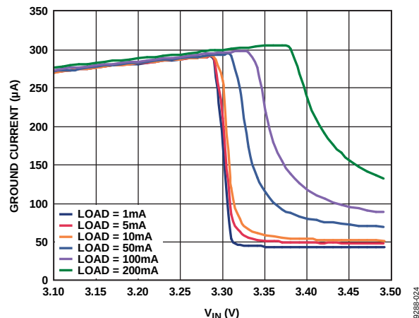
Figure 26. Ground Current vs. Input Voltage (in Dropout), V_{\text{OUT1}} = 3.3 \text{ V} , V_{\text{RIPPLE}} = 50 \text{ mV} , C_{\text{OUT}} = 1 \mu\text{F}
