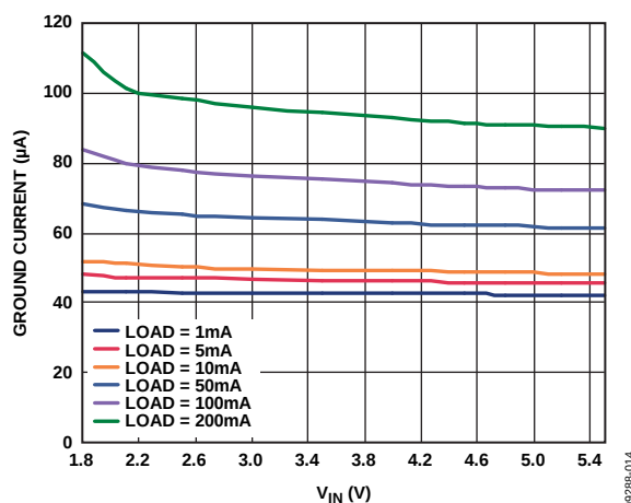
Figure 16. Ground Current vs. Input Voltage, Single Output Loaded, V_{RIPPLE} = 50\text{ mV} , C_{OUT} = 1\text{ }\mu\text{F}
