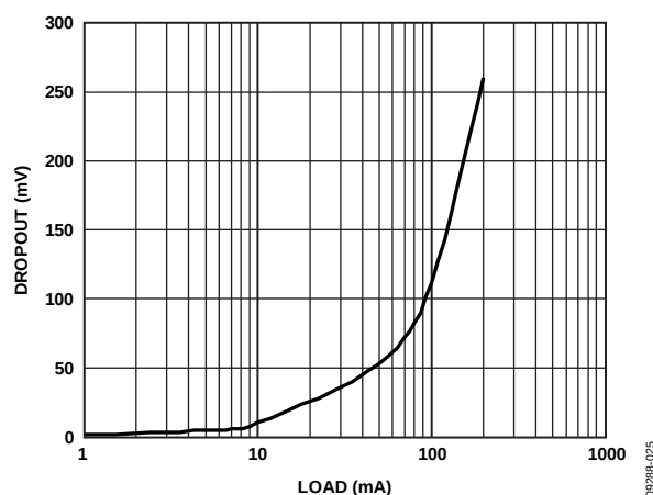
Figure 27. Dropout Voltage vs. Load Current and Output Voltage, V_{\text{OUT2}} = 1.8 \text{ V} , V_{\text{RIPPLE}} = 50 \text{ mV} , C_{\text{OUT}} = 1 \mu\text{F}
