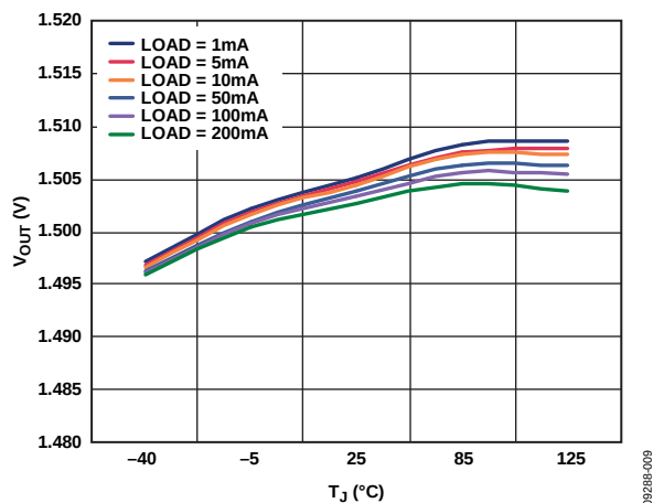
Figure 11. Output Voltage vs. Junction Temperature, V_{RIPPLE} = 50\text{ mV} , C_{OUT} = 1\text{ }\mu\text{F}
