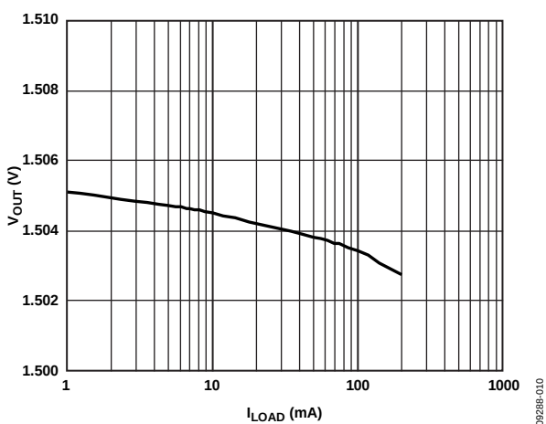
Figure 12. Output Voltage vs. Load Current, V_{RIPPLE} = 50\text{ mV} , C_{OUT} = 1\text{ }\mu\text{F}
