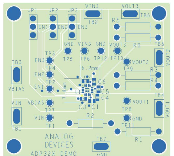
Figure 62. Example of PCB Layout, Top Side
