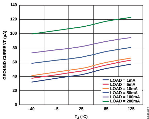
Figure 14. Ground Current vs. Junction Temperature, Single Output Loaded, V_{RIPPLE} = 50\text{ mV} , C_{OUT} = 1\text{ }\mu\text{F}
