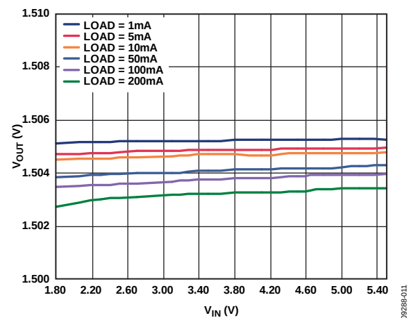
Figure 13. Output Voltage vs. Input Voltage, V_{RIPPLE} = 50\text{ mV} , C_{OUT} = 1\text{ }\mu\text{F}
