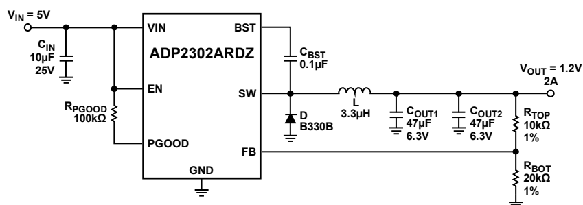
Figure 63. ADP2302 Typical Application, V_{IN} = 5\text{ V} , V_{OUT} = 1.2\text{ V} , 2\text{ A}
