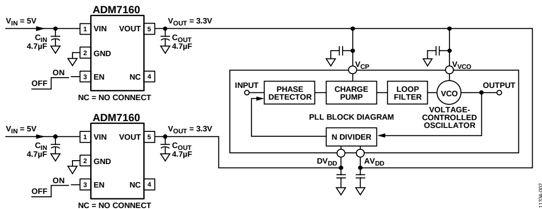
Figure 60. ADM7160 Powering a PLL/VCO
