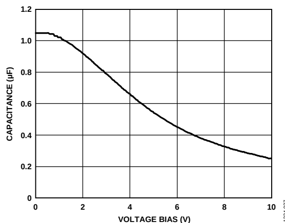
Figure 40. Capacitance vs. Voltage Bias Characteristics
