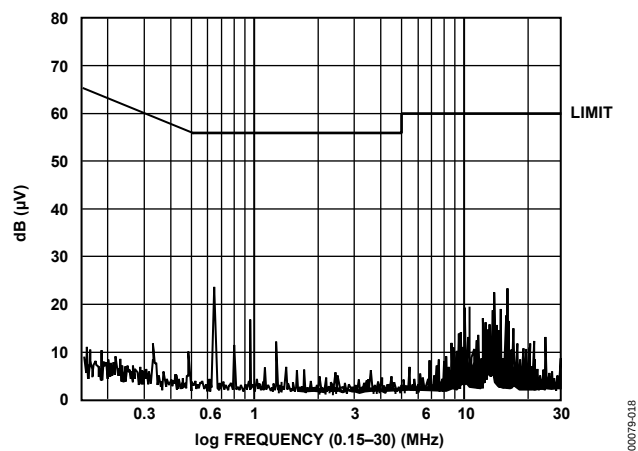
Figure 23. Conducted Emissions
