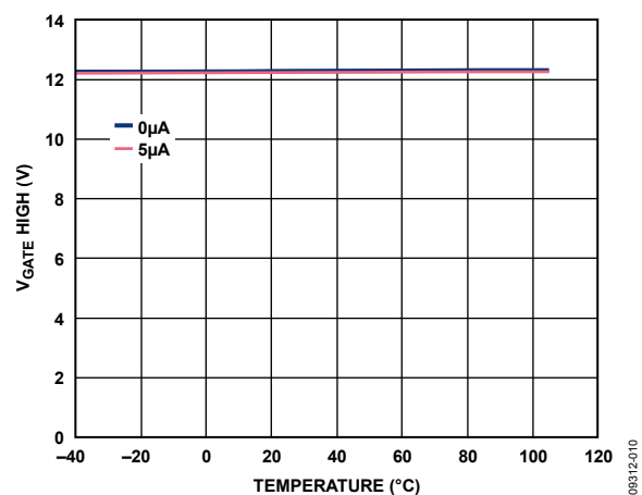
Figure 10. V_{GATE\text{ High}} vs. Temperature
