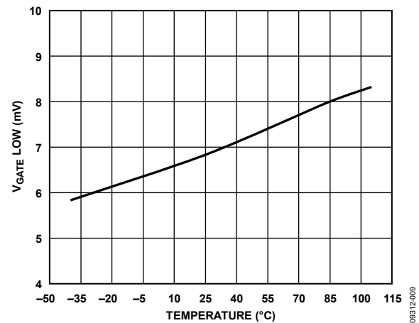
Figure 9. V_{GATE\text{ Low}} vs. Temperature ( I_{GATE} = 100\text{ }\mu\text{A} )
