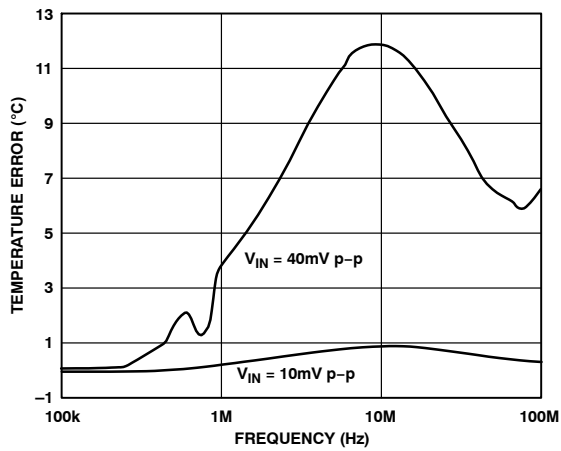
Figure 5. Temperature Error vs. Differential Mode Noise Frequency
