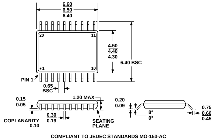
Figure 13. 20-Lead Thin Shrink Small Outline Package [TSSOP] (RU-20) Dimensions shown in millimeters
