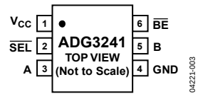
Figure 3. 6-Lead SOT-66
