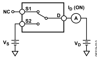
Figure 28. On Leakage
