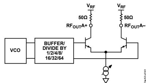
Figure 27. Output Stage
