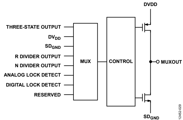
Figure 25. MUXOUT Schematic
