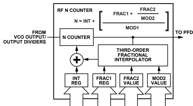
Figure 23. RF N Divider
