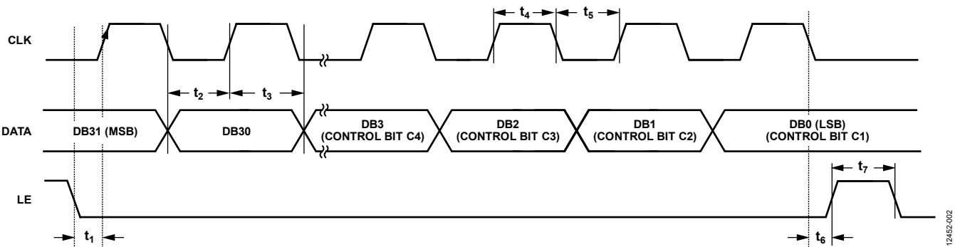
Figure 2. Timing Diagram
