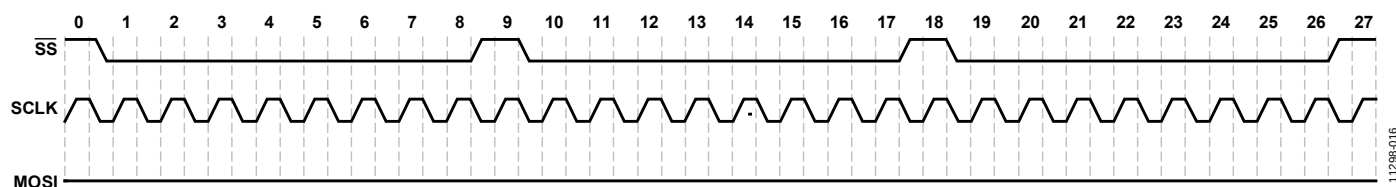
Figure 16. SPI Mode Initial Sequence
