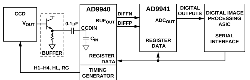
Figure 6. Typical System Block Diagram
