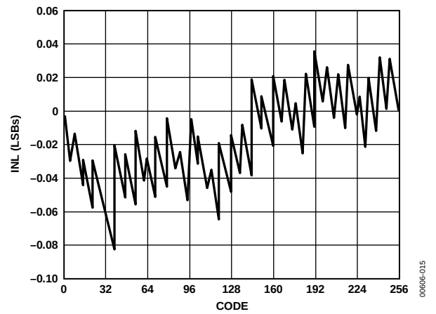
Figure 14. Typical INL
