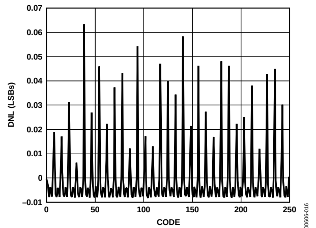
Figure 15. Typical DNL
