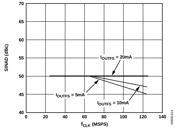
Figure 13. SINAD vs. f_{CLK} and I_{OUTFS} @ f_{OUT} = 5 MHz and 0 dBFS
