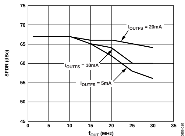
Figure 9. SFDR vs. f_{OUT} and I_{OUTS} @ 65 MSPS and 0 dBFS
