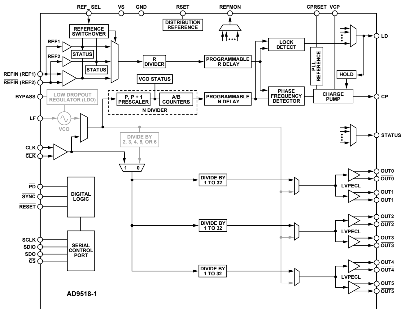
Figure 30. Clock Distribution of External VCO \leq 1600 MHz
