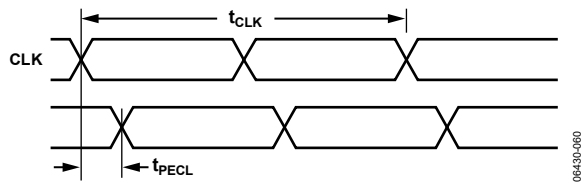
Figure 2. CLK/CLK to Clock Output Timing, DIV = 1
