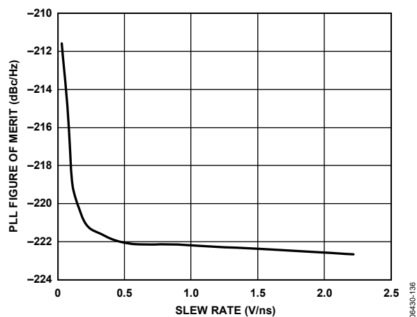
Figure 10. PLL Figure of Merit (FOM) vs. Slew Rate at \overline{REF\_IN}/\overline{REF\_IN}
