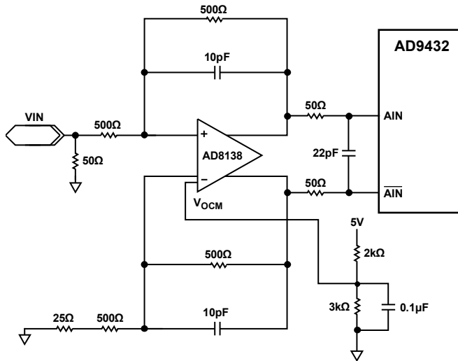
Figure 29. AD8138/AD9432 Schematic
