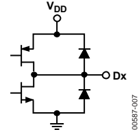
Figure 24. Digital Output Circuit
