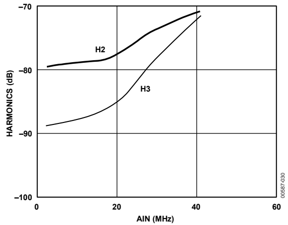
Figure 31. Measured Second-Order and Third-Order Harmonic Distortion (Encode = 105 MSPS)
