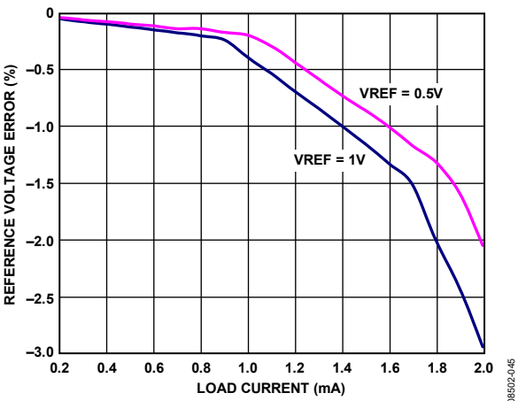
Figure 72. VREF Accuracy vs. Load
