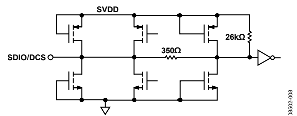
Figure 58. Equivalent SDIO/DCS Circuit
