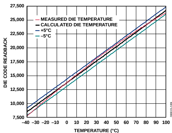
Figure 90. Die Temperature vs. Die Temperature Code Readback
