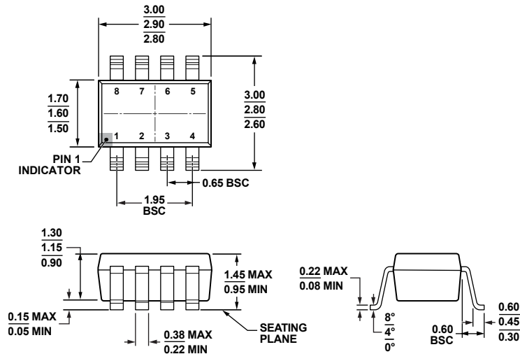
COMPLIANT TO JEDEC STANDARDS MO-178-BA Figure 40. 8-Lead Small Outline Transistor Package [SOT-23] (RJ-8) Dimensions shown in millimeters
