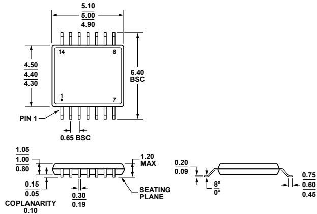
COMPLIANT TO JEDEC STANDARDS MO-153-AB-1 Figure 41. 14-Lead Thin Shrink Small Outline Package [TSSOP] (RU-14) Dimensions shown in millimeters
