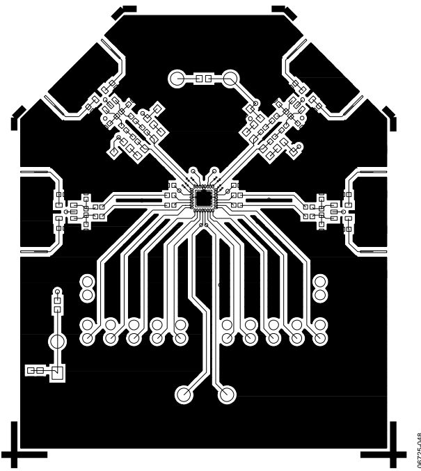
Figure 50. Component Side Layout
