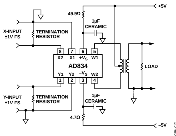
Figure 16. Transformer-Coupled Output
