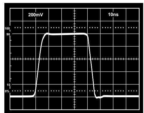
Figure 19. Pulse Response for the Circuit of Figure 18
