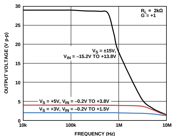
Figure 27. Large Signal Frequency Response
