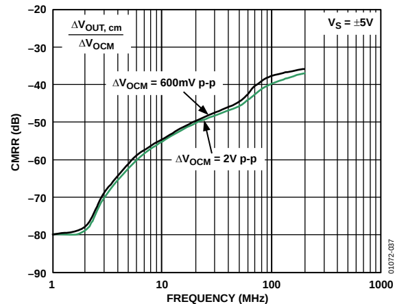
Figure 37. V_{OCM} CMRR vs. Frequency
