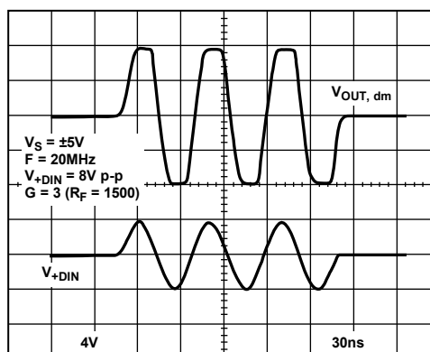
Figure 26. Output Overdrive
