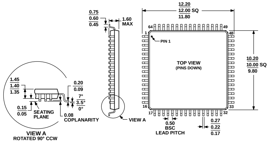
Figure 40. 64-Lead Low Profile Quad Flat Package [LQFP] (ST-64-2) Dimensions shown in millimeters
