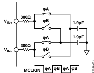
Figure 30. Analog Input Equivalent Circuit
