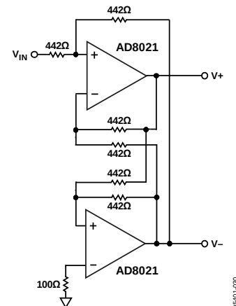
Figure 43. Single-Ended-to-Differential Configuration with the AD8021
