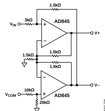
Figure 42. Single-Ended-to-Differential Configuration with the AD845
