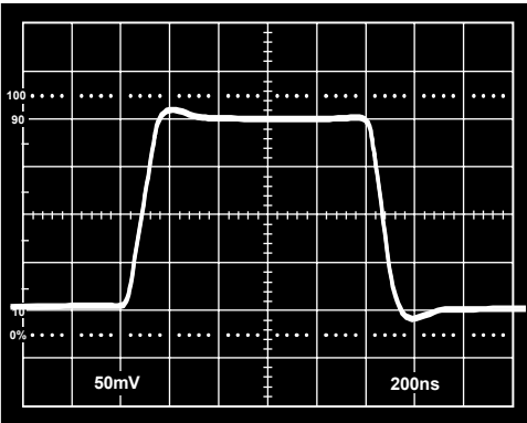
Figure 28. Unity-Gain Inverter Pulse Response (Small Signal)
