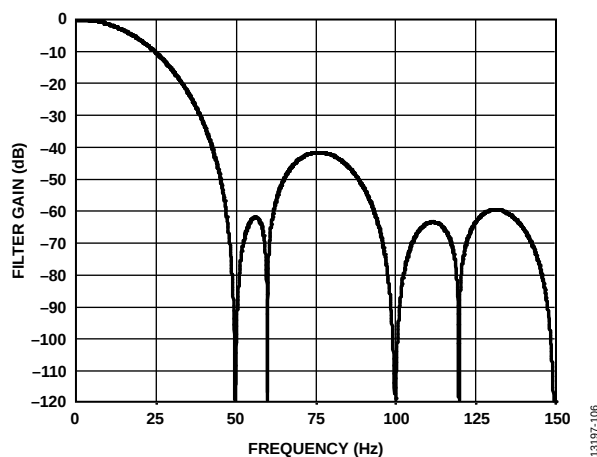
Figure 100. Sinc 3 Filter Response (50 SPS Output Data Rate, Zero Latency Disabled or 16.67 SPS Output Data Rate, Zero Latency Enabled, REJ60 = 1)
