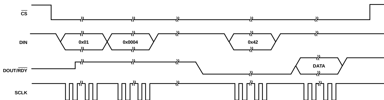
Figure 82. Single Conversion Configuration
