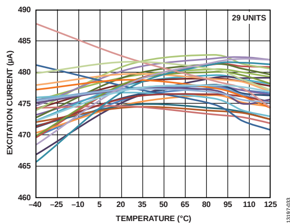
Figure 33. Excitation Current Drift (500 \mu A)
