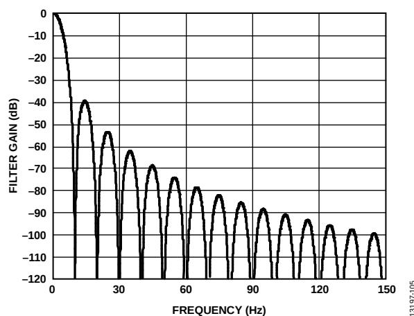
Figure 99. Sinc 3 Filter Response (10 SPS Output Data Rate, Zero Latency Disabled or 3.33 SPS Output Data Rate, Zero Latency Enabled)
