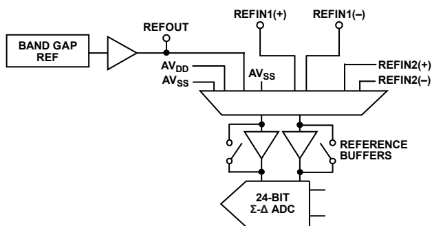
Figure 79. Reference Connections
