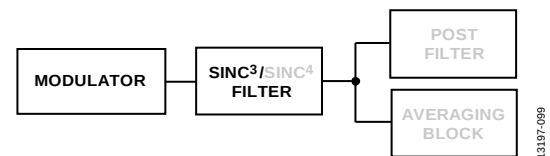
Figure 93. Sinc 3 Filter
