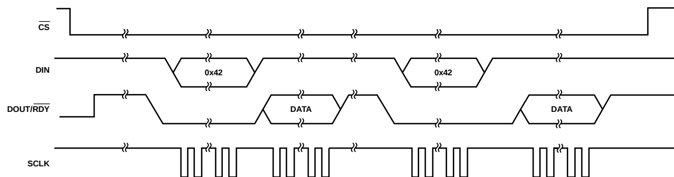
Figure 83. Continuous Conversion Configuration
