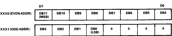
Figure 14. AD574A Data Format for 8-Bit Bus
