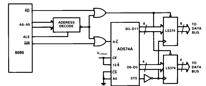
Figure 13. 8086 Stand-Alone Configuration
