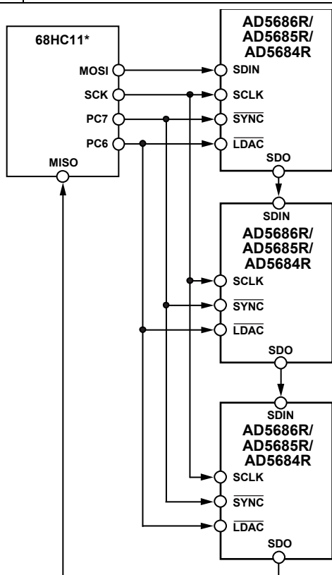
*ADDITIONAL PINS OMITTED FOR CLARITY. Figure 53. Daisy-Chaining the AD5686R/AD5685R/AD5684R
