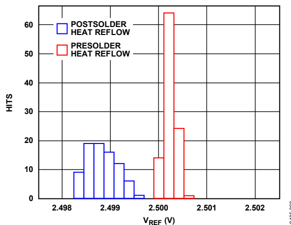
Figure 56. SHR Reference Voltage Shift
