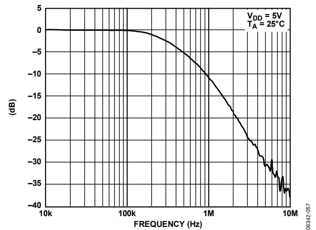
Figure 51. Multiplying Bandwidth
