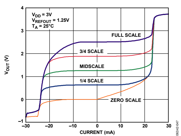
Figure 35. AD5627R/AD5647R/AD5667R with 1.25\text{V} Reference, Source and Sink Capability
