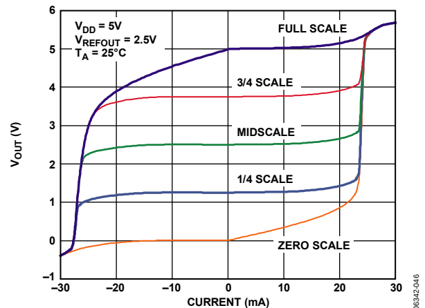
Figure 34. AD5627R/AD5647R/AD5667R with 2.5\text{V} Reference, Source and Sink Capability
