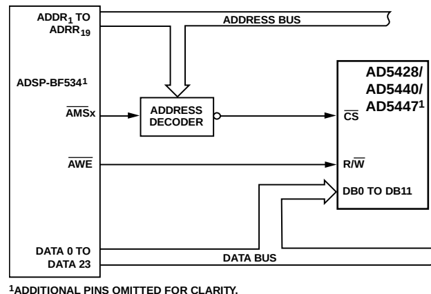
Figure 45. ADSP-BF534-to-AD5428/AD5440/AD5447 Interface
