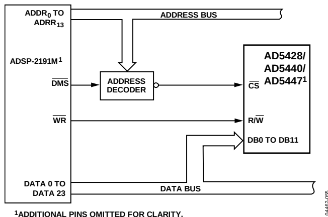
Figure 43. ADSP-2191M-to-AD5428/AD5440/AD5447 Interface
