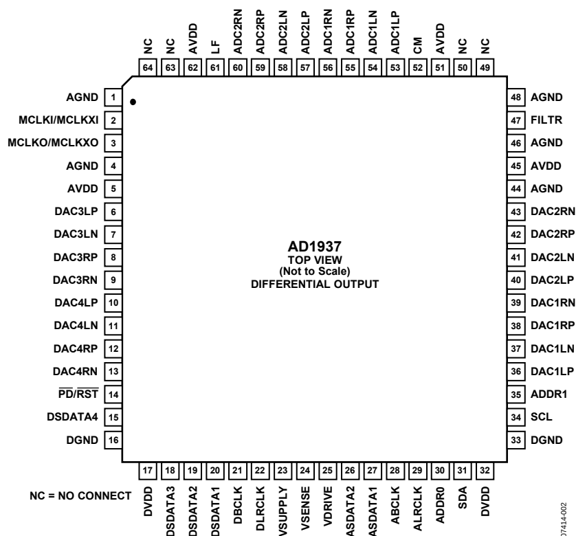
Figure 4. Pin Configuration
