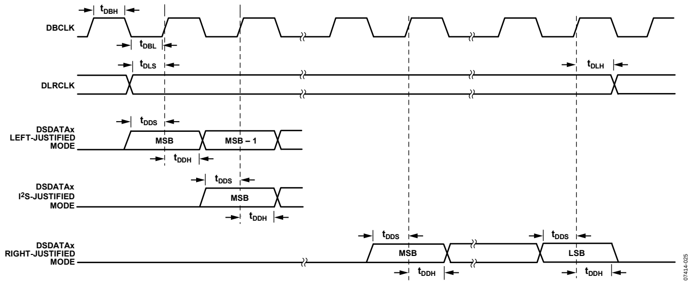
Figure 2. DAC Serial Timing
