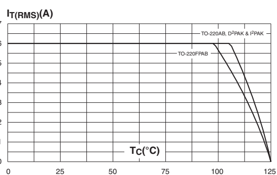
Figure 5: RMS on-state current versus case temperature (full cycle)
