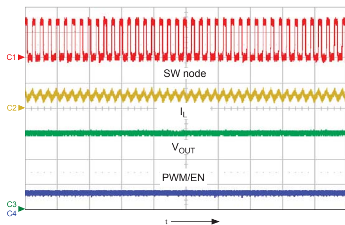
Figure 25. Normal operation of the switch node (SW); inductor current ( I_L ) and output voltage ( V_{OUT} ) for 9 series LEDs in each of four strings configuration; shows SW node (ch1, 20 V/div.), inductor current I_L (ch2, 1 A/div.), V_{OUT} (ch3, 10 V/div.), and PWM/EN (ch4, 5 V/div.), time = 2 μs/div.
