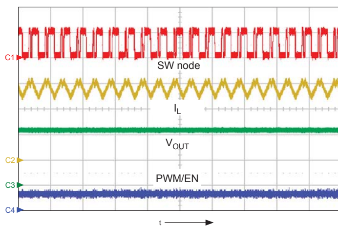
Figure 26. Cycle-by-cycle current limiting; inductor current (yellow trace, I_L ), note reduction in output voltage as compared to normal operation with the same configuration (figure 26); shows SW node (ch1, 20 V/div.), inductor current I_L (ch2, 1 A/div.), V_{OUT} (ch3, 10 V/div.), and PWM/EN (ch4, 5 V/div.), time = 2 μs/div.
