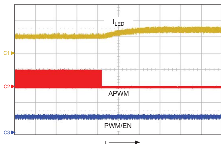
Figure 16. Diagram showing the transition of LED current from 60 mA to 80 mA, when a 25% duty cycle signal is removed from the APWM pin. PWM = 1; shows I_{LED} (ch1, 50 mA/div.), APWM (ch2, 10 V/div.), and PWM/EN (ch3, 5 V/div.), time = 500 \mu s/div.
