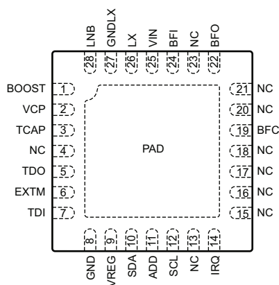
Pinout Diagram
