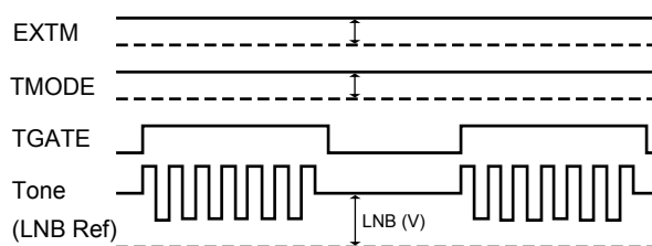
Option 1 – Use internal tone, gated by the TGATE bit.
