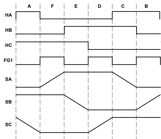
DIR = 0 = Reverse
