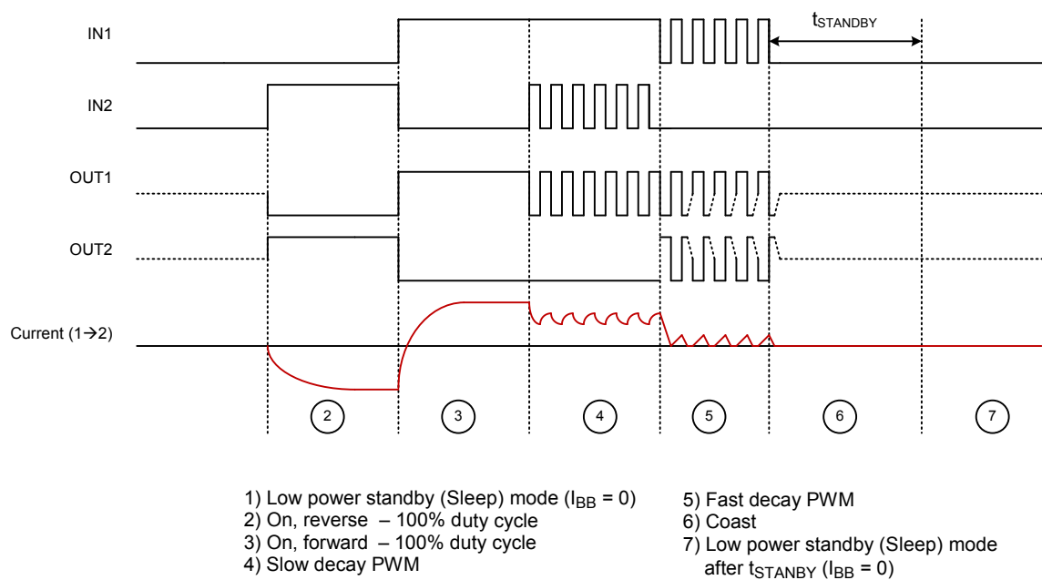
DC Motor Timing Diagram
