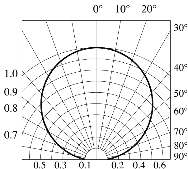
Fig.6 - Radiation Diagram
